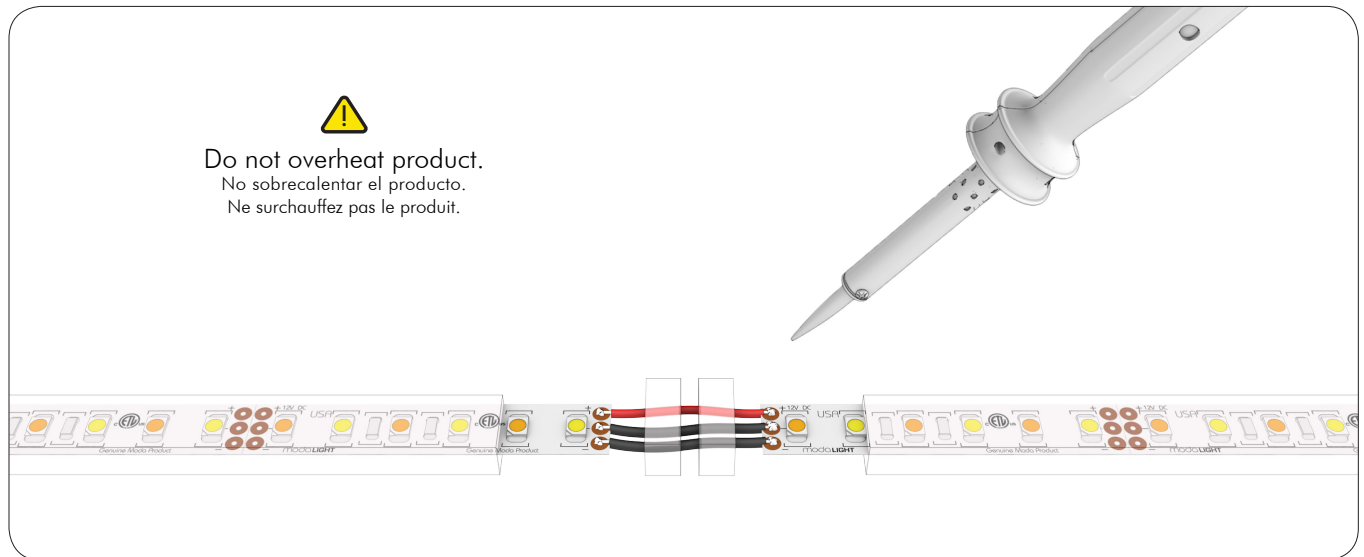
Solder connection
