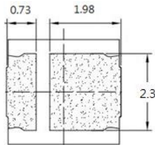
Soldering Pad Pattern
