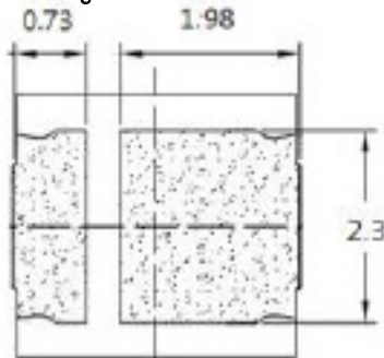
Soldering Pad Pattern
