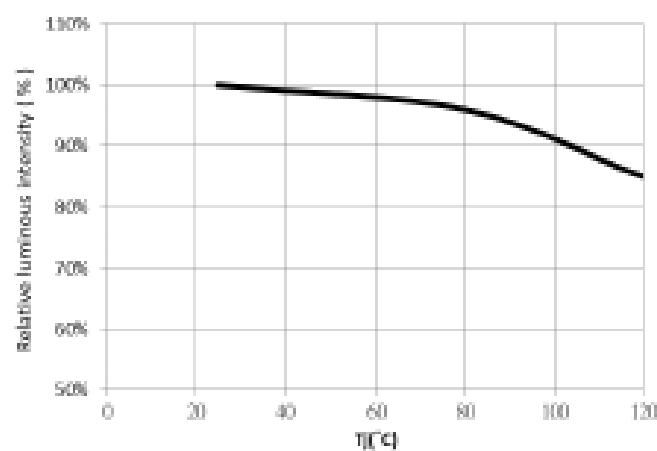
Relative Luminous vs. Ambient Temperature
