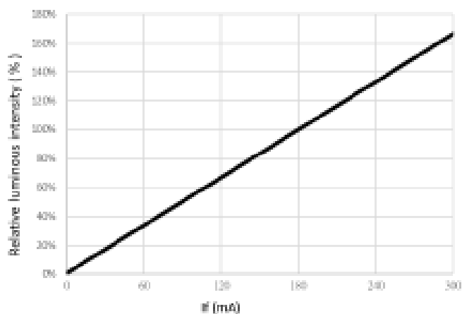
Relative Luminous vs. Forward Current
