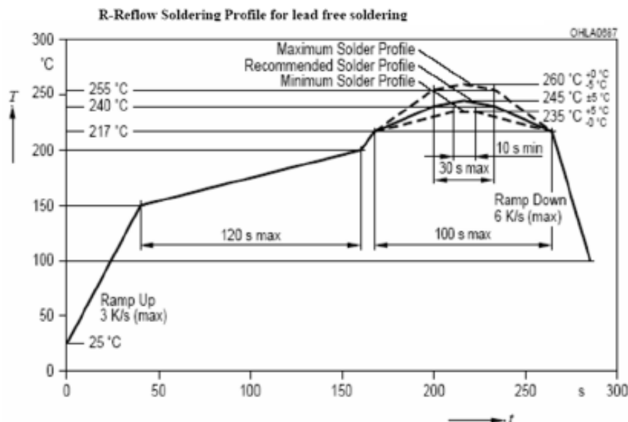
Recommended Reflow Conditions
